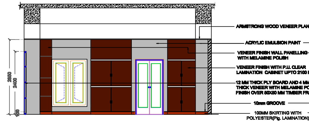
ELEVATION C
