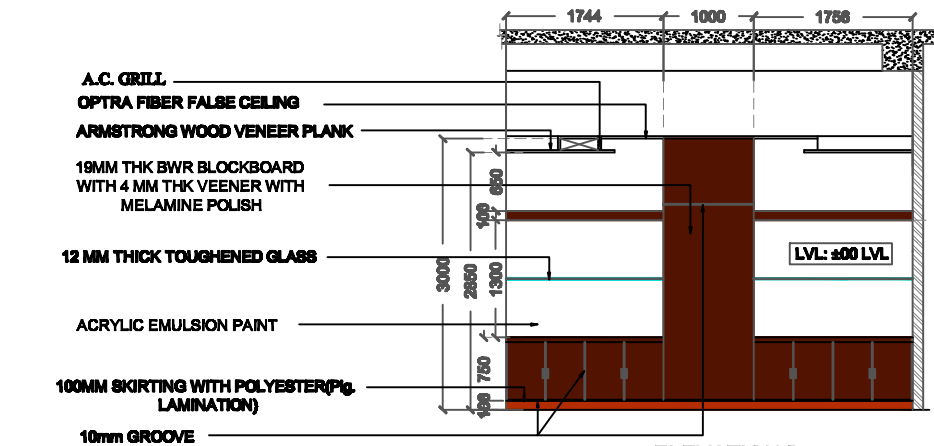
ELEVATION D
