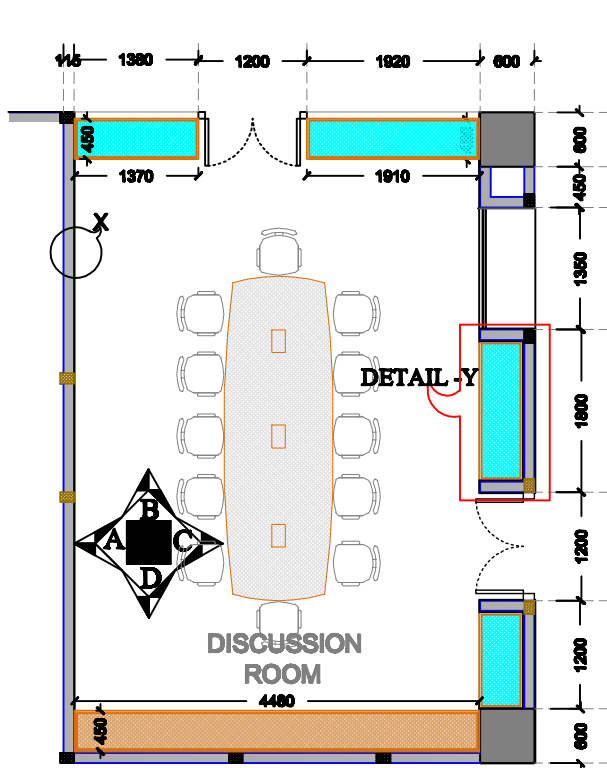
FURNITURE LAYOUT PLAN
