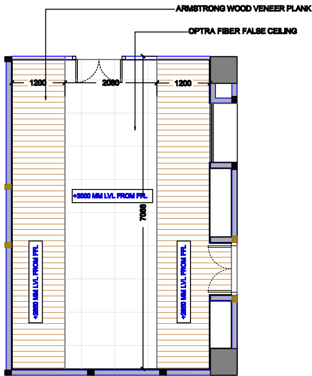
REFLECTED CEILING PLAN LAYOUT
